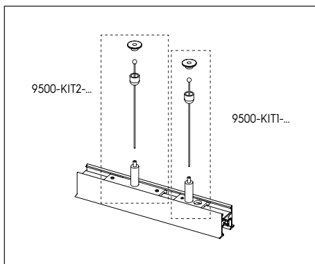
吊线组件 Complete suspension kit
